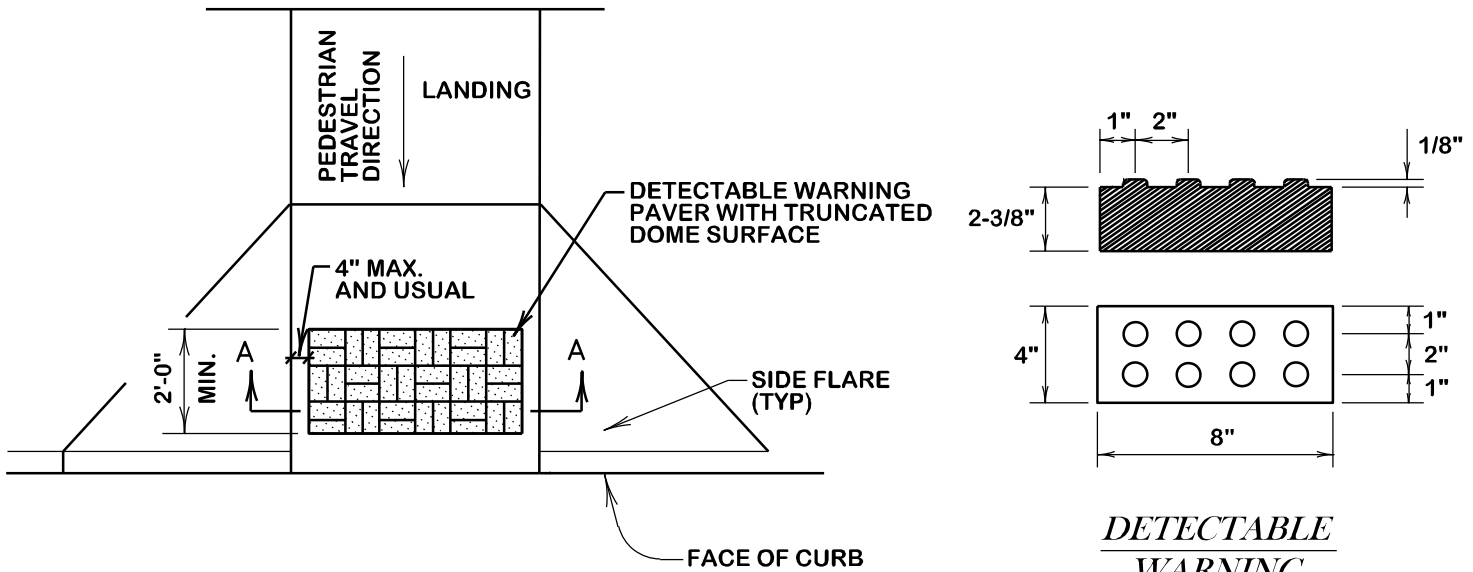
TRUNCATED DOME PATTERN CURB RAMP
