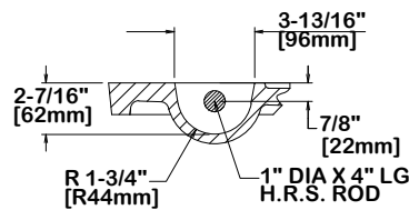
PICKBAR DETAIL
