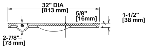
COVER SECTION
