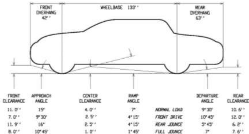
COMPOSITE LONGEST VEHICLE: CLEARANCE DIMENSIONS UNDER VARIOUS CONDITIONS
