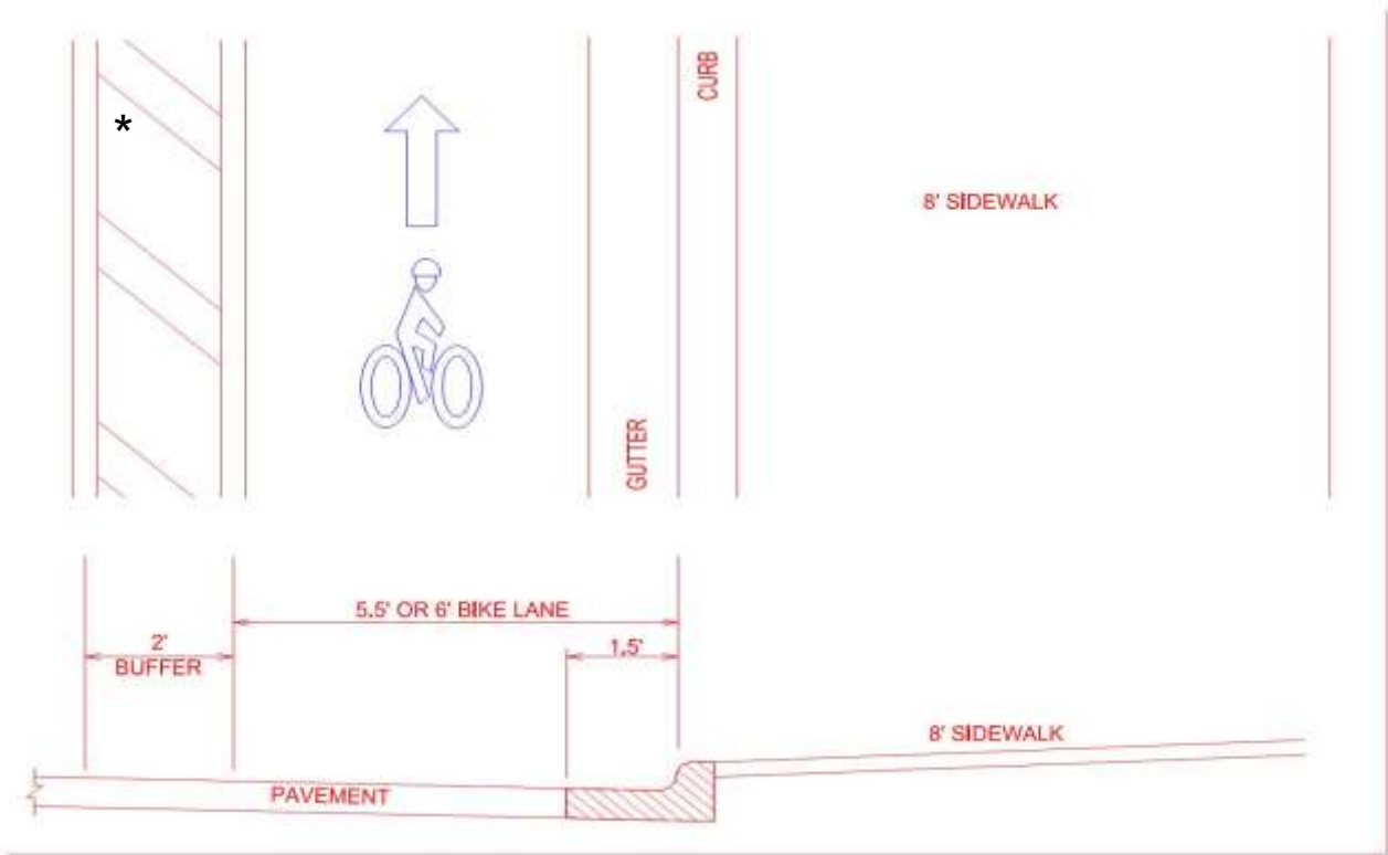
FIGURE 5 BIKE LANE DIAGRAM
