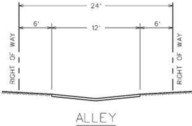
FIGURE 1 RESIDENTIAL STREET SECTIONS
