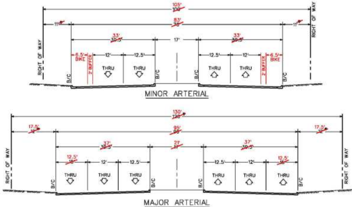
FIGURE 3 ARTERIAL STREET SECTIONS
