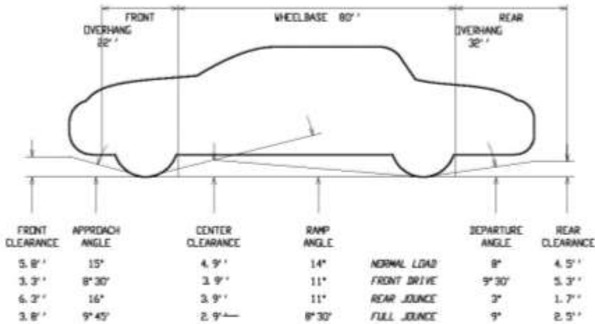
COMPOSITE SHORTEST VEHICLE: CLEARANCE DIMENSIONS UNDER VARIOUS CONDITIONS
