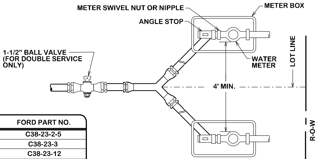
VIEW A-A DOUBLE SERVICE
