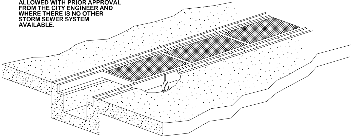
ISOMETRIC VIEW
